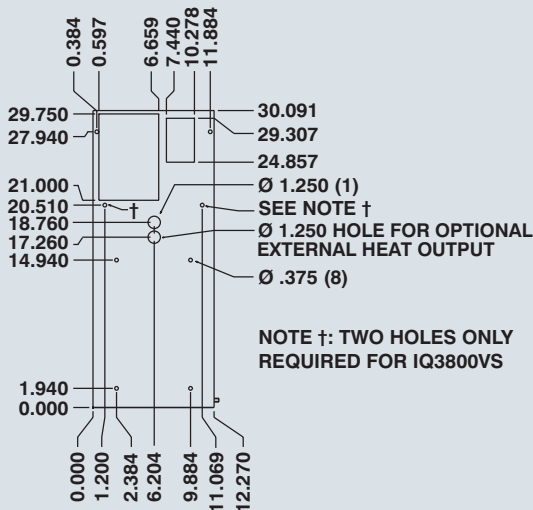
CUT-OUT DRAWING
