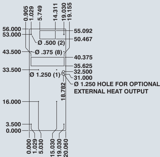
CUT-OUT DRAWING
