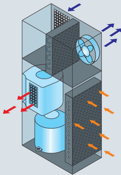
CUT-OUT DRAWING
