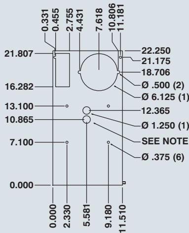
CUT-OUT DRAWING
