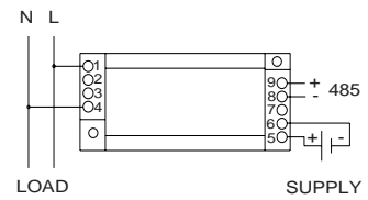
CRD4510 VOLTAGE TRANSDUCER
