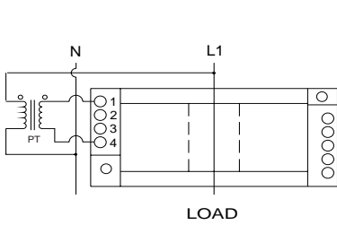
Single Phase
