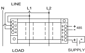
CRD5150 MULTIFUNCTION TRANSDUCER
