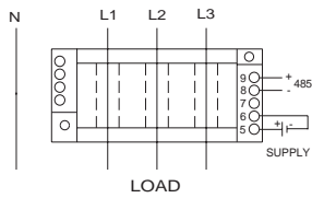
CRD4170 CURRENT TRANSDUCER
