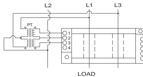
3 Phase 3-Wire
